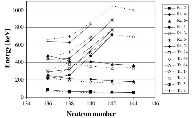
Fig. 4. Systematics of the first-excited states in K^\pi = 0^+ ( J = 2, 4 and 6 ) and 0^- bands in even-even Ra and Th isotopes.
