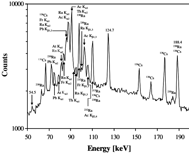
Fig. 2. Beta-delayed ^{232}\text{Fr} gamma-spectrum accumulated during the experiment.
