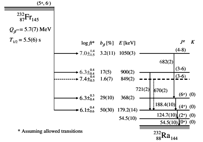
Fig. 3. A suggested beta-decay scheme for ^{232}\text{Fr} . Due to the low statistics, the transition marked with a dashed arrow should be treated with some caution.
